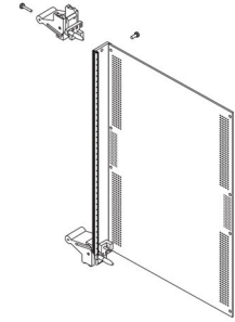
6U Front Panel Assembly (with Injector/Ejector Handles)
