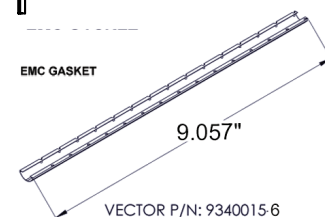
VECTOR P/N: 9340015-6 MATERIAL: STEEL WITH BRIGHT NICKEL FINISH
